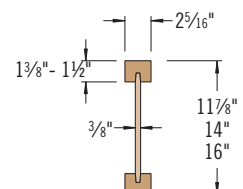
TJI® 360 joists
