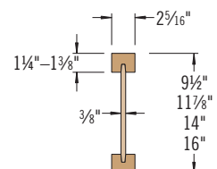
TJI® 230 joists
