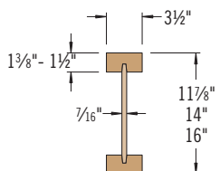
TJI® 560 joists
